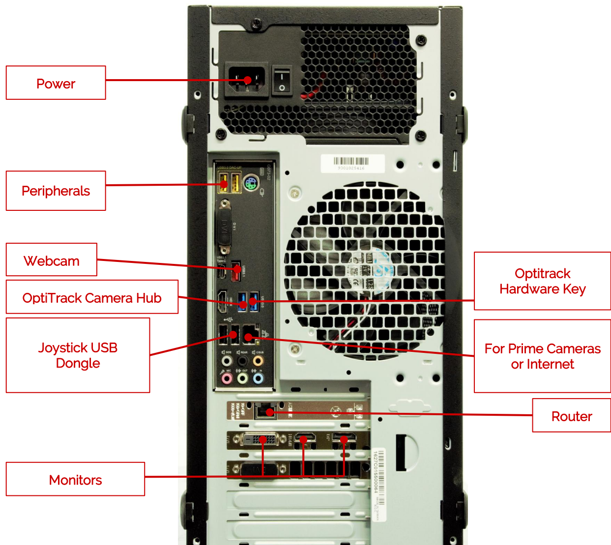
Figure 1: PC wiring
