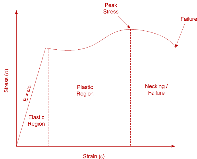
Figure 2: Stress-strain curve
