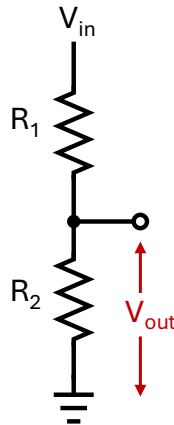
Figure 2: Voltage divider circuit
