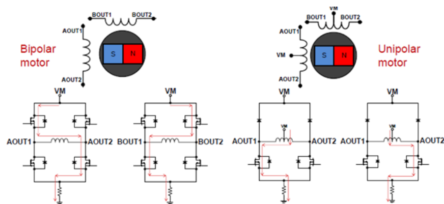
Figure 4: Unipolar and bipolar stepper motor circuits
