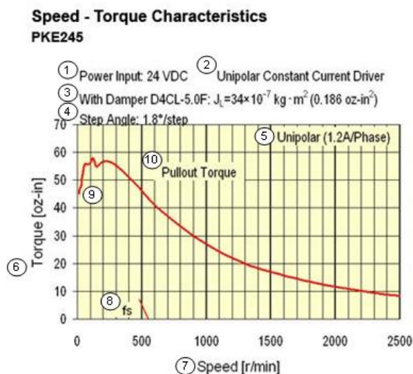
Figure 10: Speed-torque curve for a stepper motor
