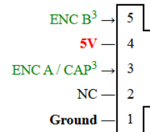
Encoder Connector
