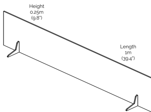
Figure 17: QBot System walls with dimensions
