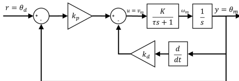
Figure 7. Block diagram of proportional plus rate feedback control
