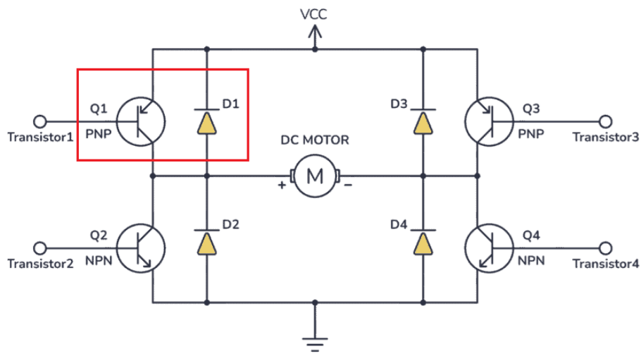
Figure 6. H bridge to help drive a motor. The circuit in red acts like a switch.
