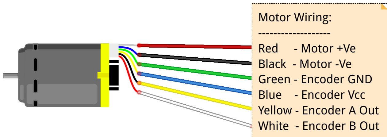
Figure 4: Typical brushed DC motor wire connections and color coding
