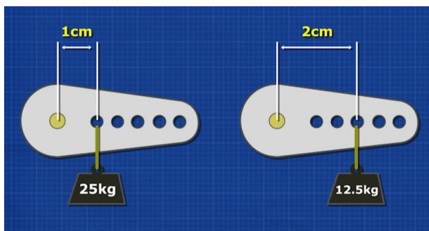
Figure 5. Motor Torque measured in kg/cm
