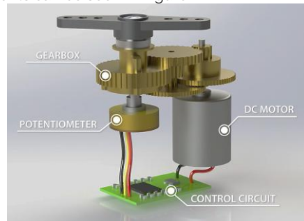
Figure 1. Internal Layout of a Servomotor
