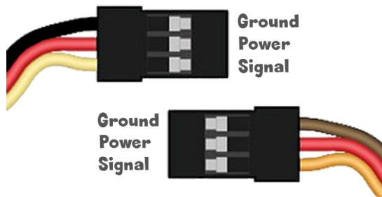
Figure 2. Hobby Servomotors Wiring Connector
