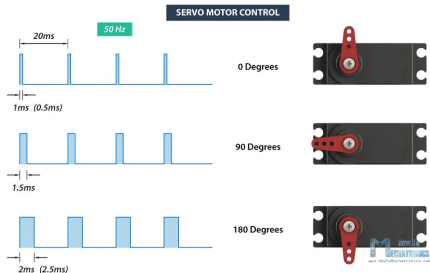
Figure 3. Control Signal for a Servomotor
