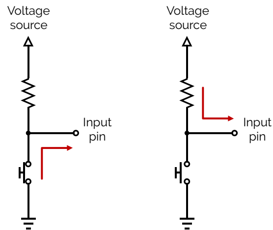
Figure 3: Push button connected with pull-up resistor, in closed and open states
