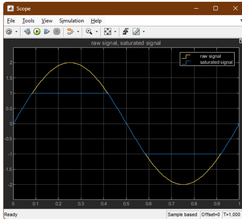
Figure 1. a sinusoid input (yellow) with an amplitude of 2 passes through a saturation set to a maximum amplitude of 1.
