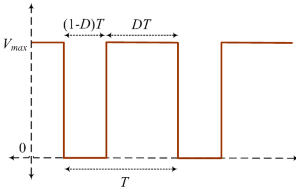
Figure 3: A pulse waveform
