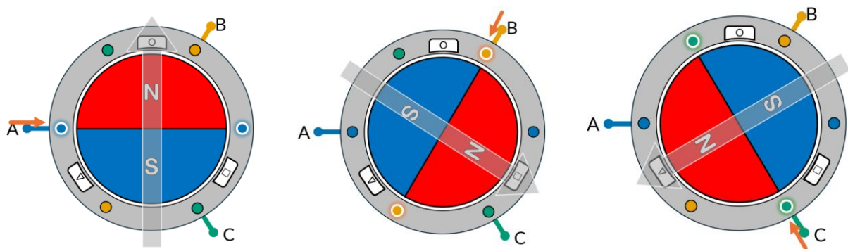
Figure 4. Magnet positions and magnetic fields when energizing coils
