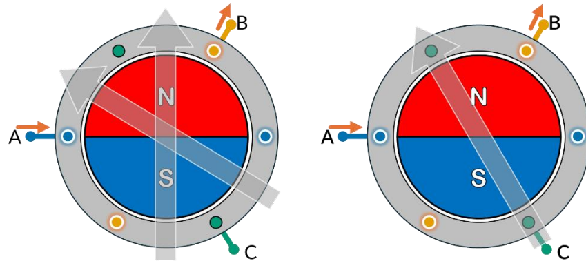
Figure 8. Magnetic Fields from Energizing 2 Coils and Equivalent Magnetic Field
