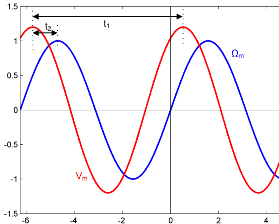
Figure 5. Period and phase delay of sinusoidal signals
