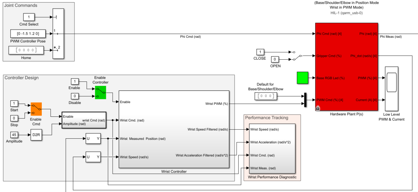
Figure 4: Simulink model that controls the QArm in hybrid Position/PWM Mode.
