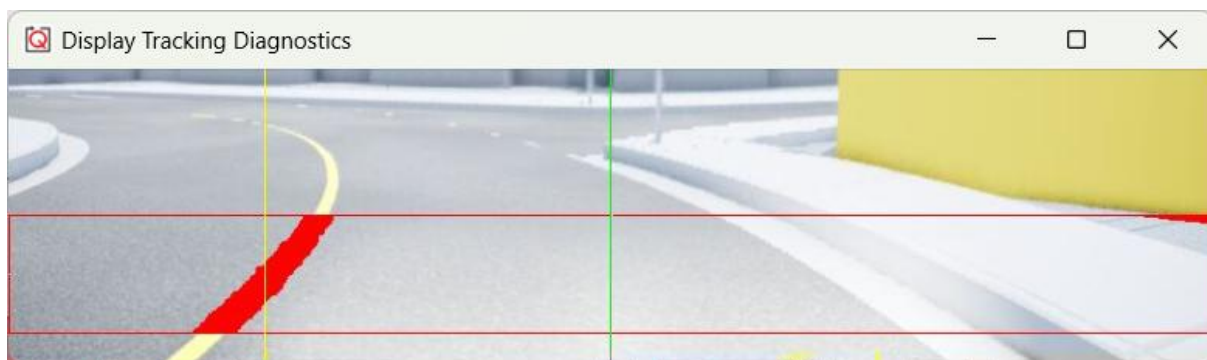
Figure 3. Processed lane extraction Image.
