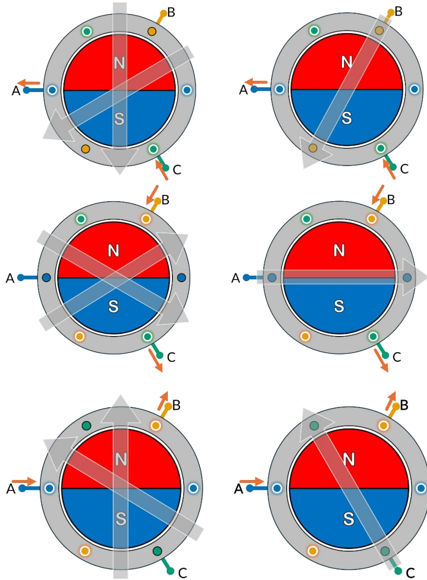
Figure 8: Magnetic fields from energizing 2 coils and equivalent magnetic field
