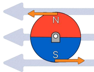
Figure 7: Magnetic field for maximum torque
