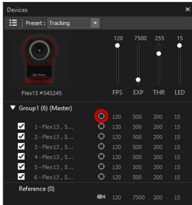
Figure 2. Devices pane in Motive: detecting cameras
