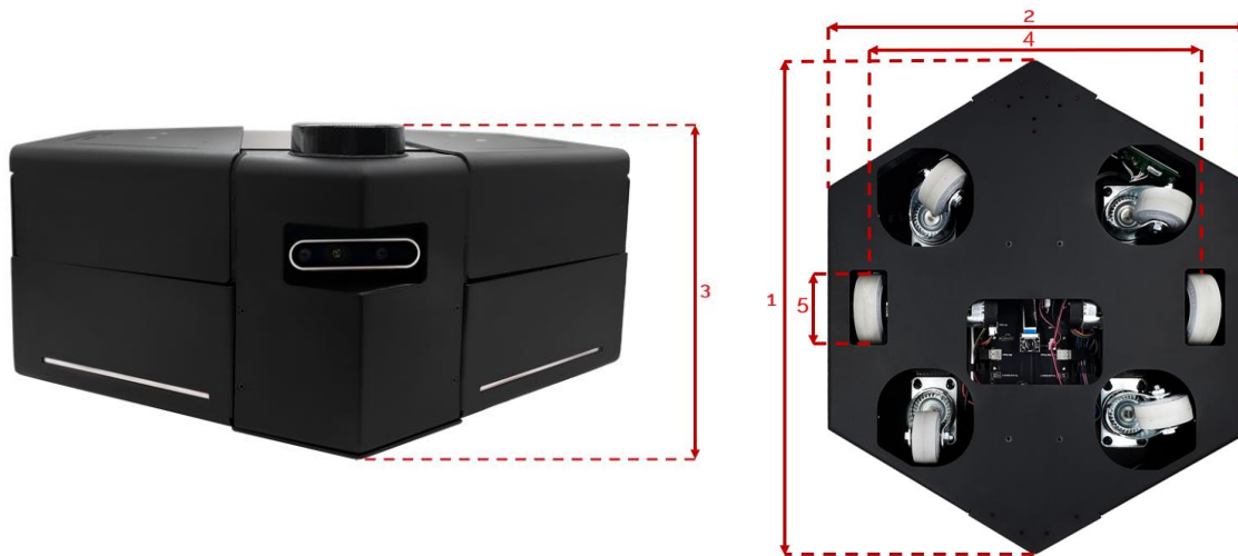
Figure 10. QBot Dimensions
