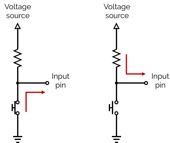
Figure 2: Push button connected with pull-up resistor, in closed and open states
