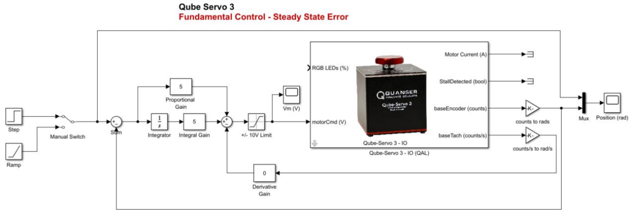
Figure 2: Simulink/QUARC model implementing PID position control.
