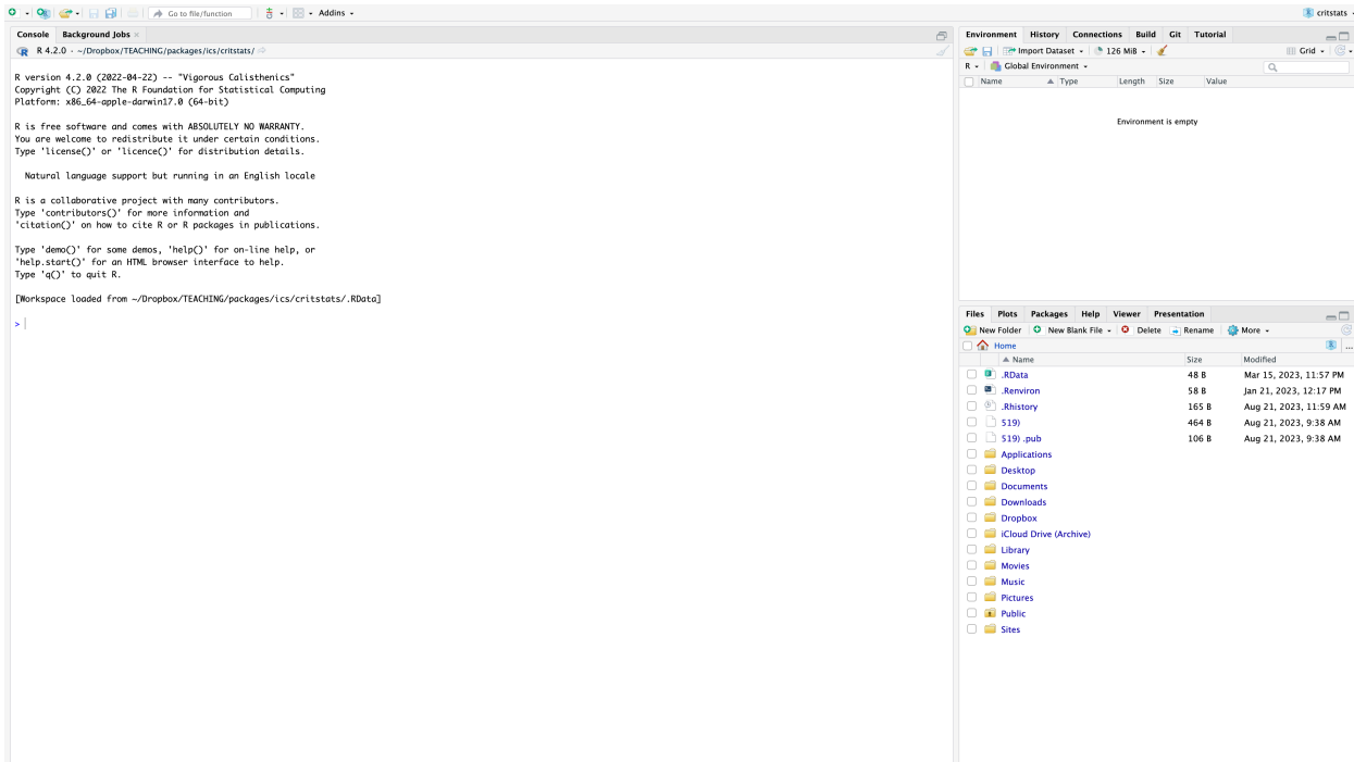
Figure 1: RStudio Panel
