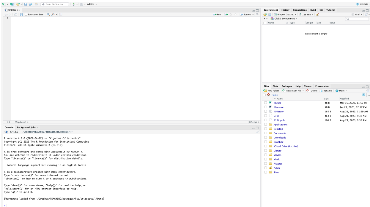
Figure 2: RStudio Panel
