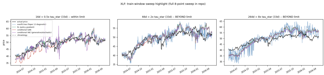
Figure 7. XLF. A visible, growing upward bias appears in the model cluster by 8x , most apparent in the 2025-10 through 2026-04 stretch, while the tree remains its own noisy, non-participating self throughout.
