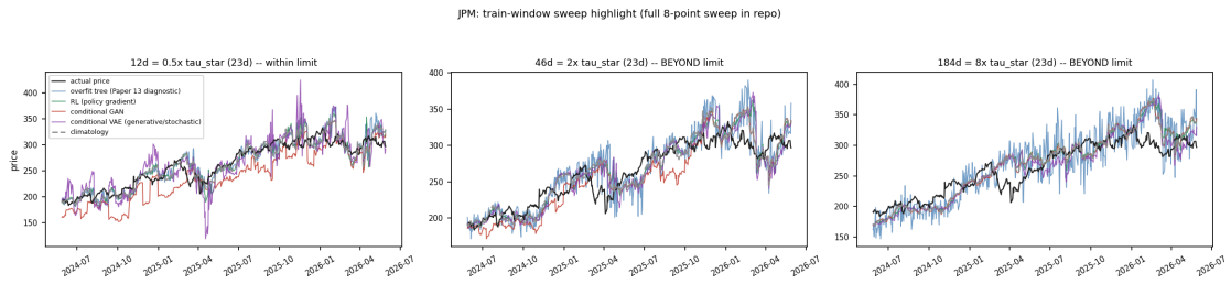
Figure 6. JPM. The same gradual detachment, building across the three panels rather than appearing discontinuously — consistent with the common-sense expectation that a real predictability limit should produce a build, not an abrupt flatline, at the boundary.
