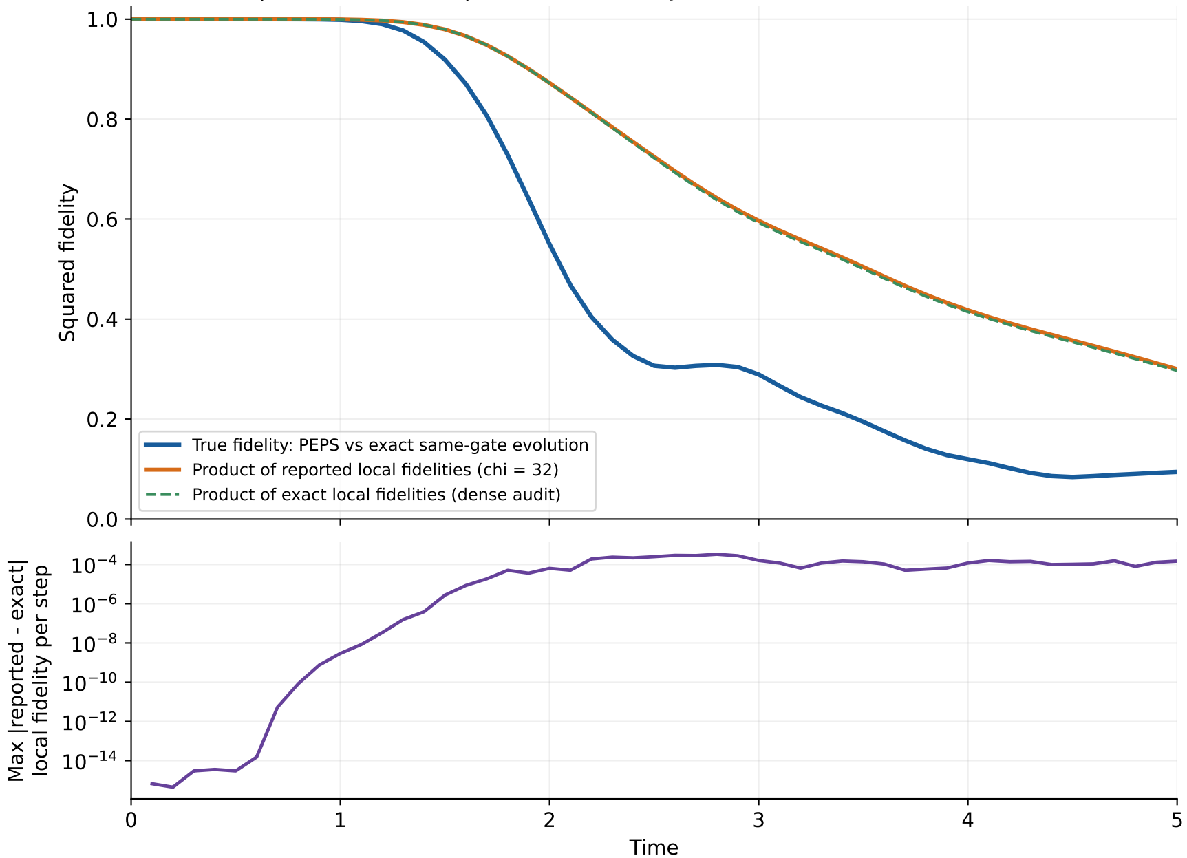
3 x 4 transverse-field Ising: PEPS D = 4, boundary \chi = 32 Open boundaries; |+\rangle initial state; J = h = 1 ; second order, dt = 0.1
