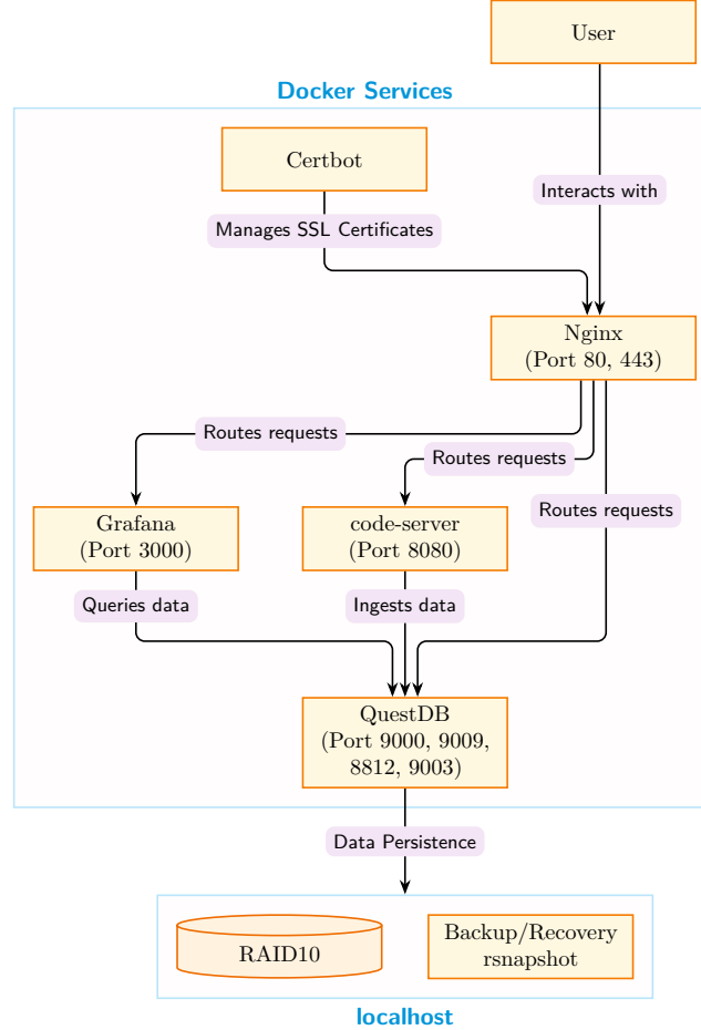
Figure 1: Network and security architecture with Nginx reverse proxy providing SSL termination and routing to containerized services.
