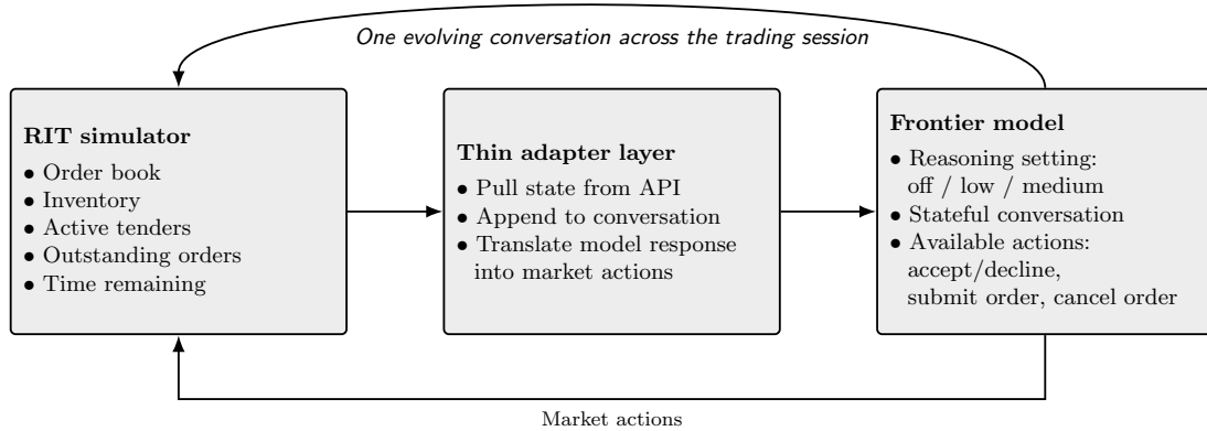
Panel B. RIT-Agent Architecture
