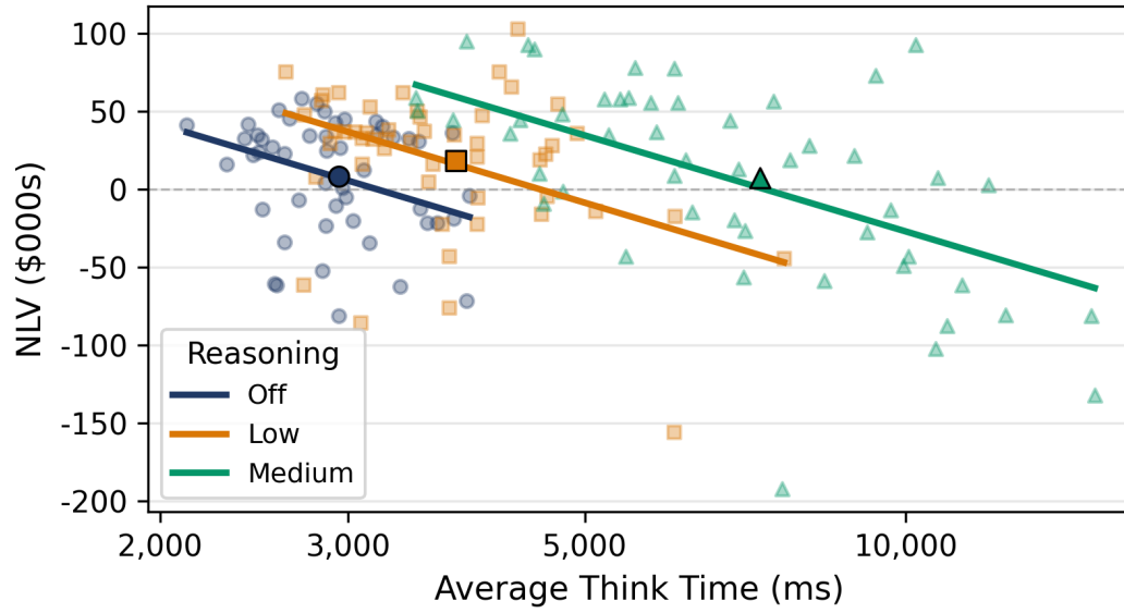
Figure 3: Session NLV vs. average think time per agent turn, gpt-5.4 in the normal-speed market ( N = 150 ). Each point is one session, colored by reasoning level. Solid lines are within-reasoning OLS fits from NLV_i = \alpha + \gamma_k \text{Reasoning}_i + \beta \ln(\text{ThinkTime}_i) + \varepsilon_i . Filled markers are cell means. Horizontal axis is log-scaled; \ln(\text{ThinkTime}) is a post-treatment variable.
