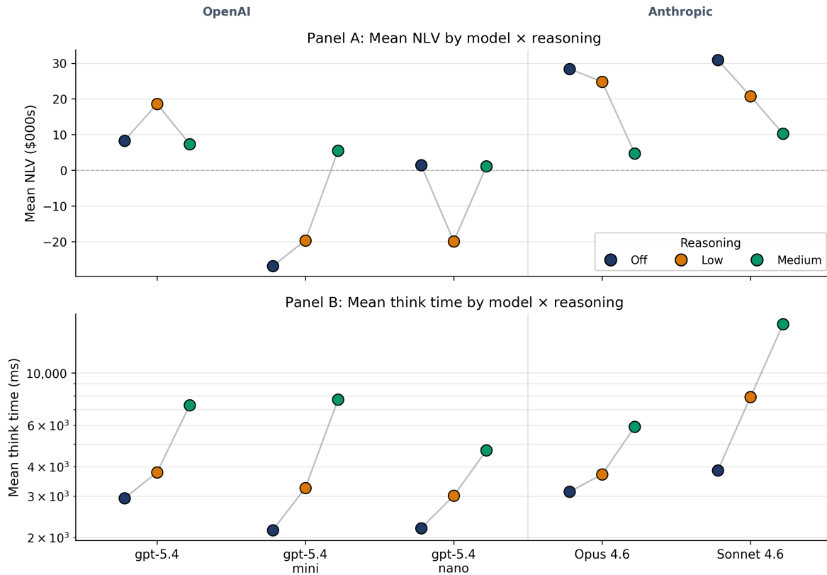
Figure 10: Connected-means view of model and reasoning (50 sessions per reasoning cell for each model; all at normal simulation speed). Panel A: mean session NLV ($000s); Panel B: mean think time per agent turn (ms, log scale). Within each model’s x-slot, three points at small horizontal offsets show mean off, low, and medium in that order, connected by a thin grey line that traces each model’s reasoning trajectory. A vertical separator divides the OpenAI family (gpt-5.4, mini, nano) from the Anthropic family (Opus 4.6, Sonnet 4.6).
