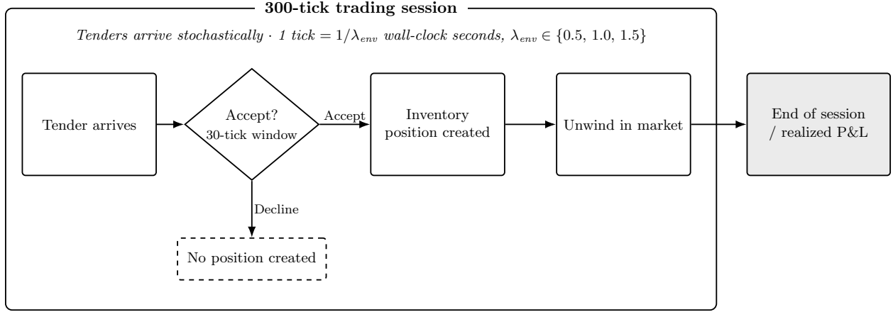
Panel A. LT3 Tender-Execution Task
