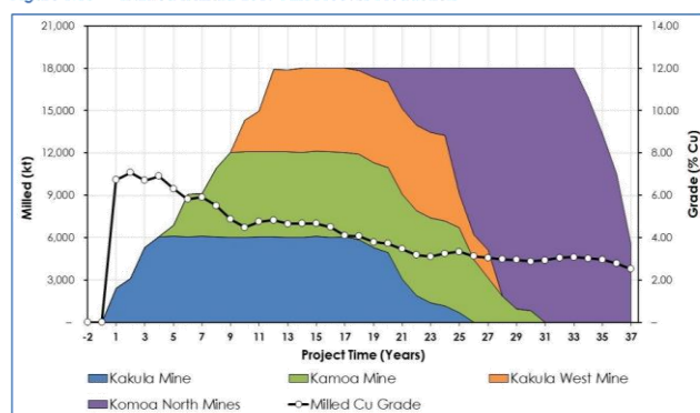
Figure 1.18 Kamo-A-Kakula 2019 PEA Process Production
