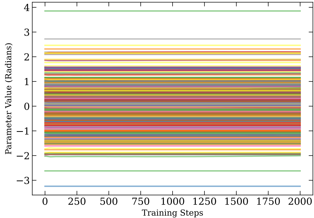
QCNN
