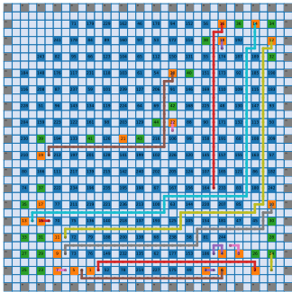
Outer 1D Double
