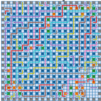
Outer 1D Projective
