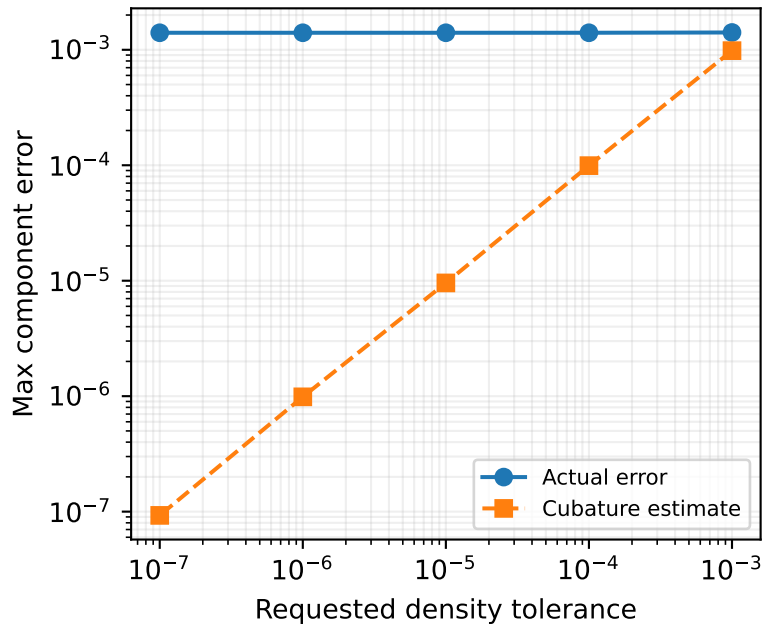
metal 2d (fixed charge mesh)
