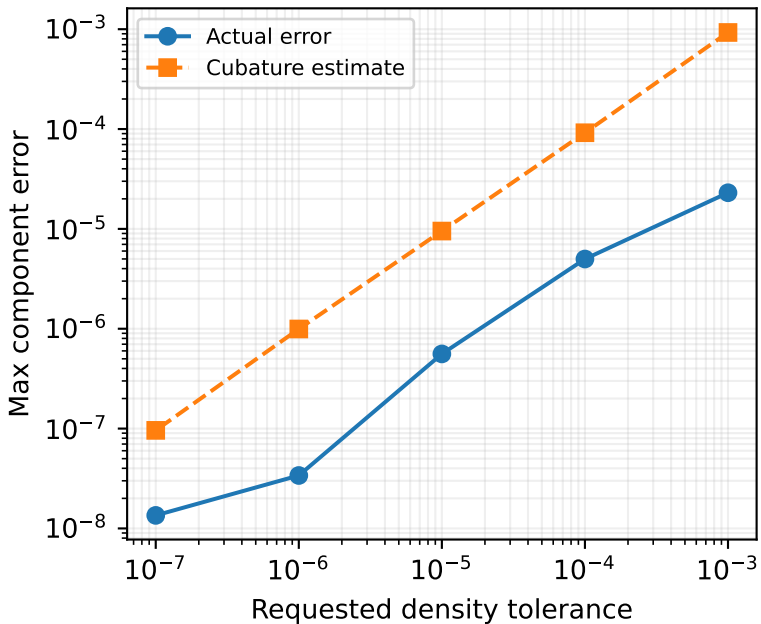
bulk 2d (fixed charge mesh)
