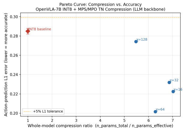
Figure 1: Compression-accuracy Pareto frontier. Lower-right is better.
