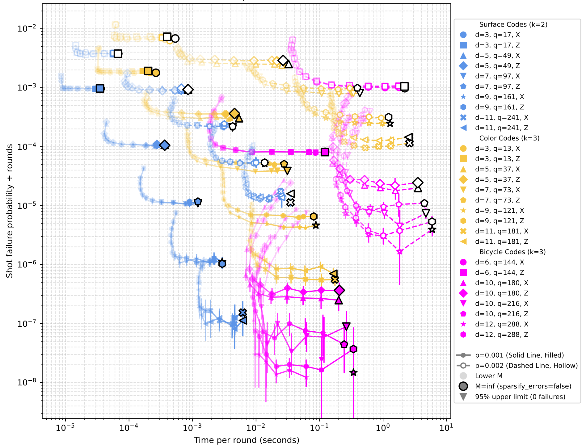
Failure Rate vs Time per Round (Combined)
