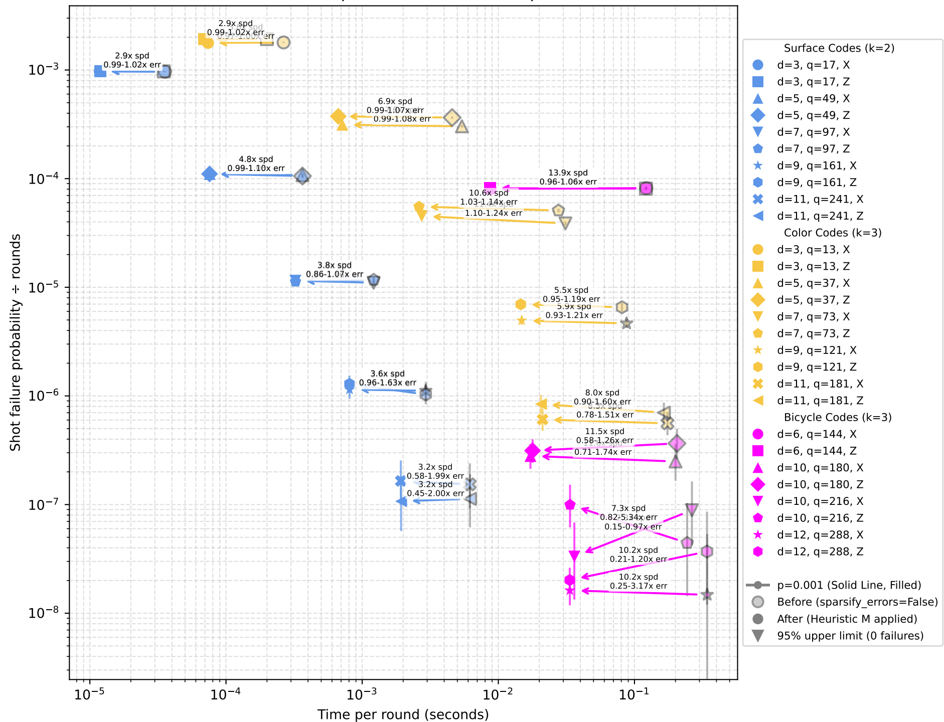
Before vs After: Sparsification Tradeoffs ( p=0.001 )
