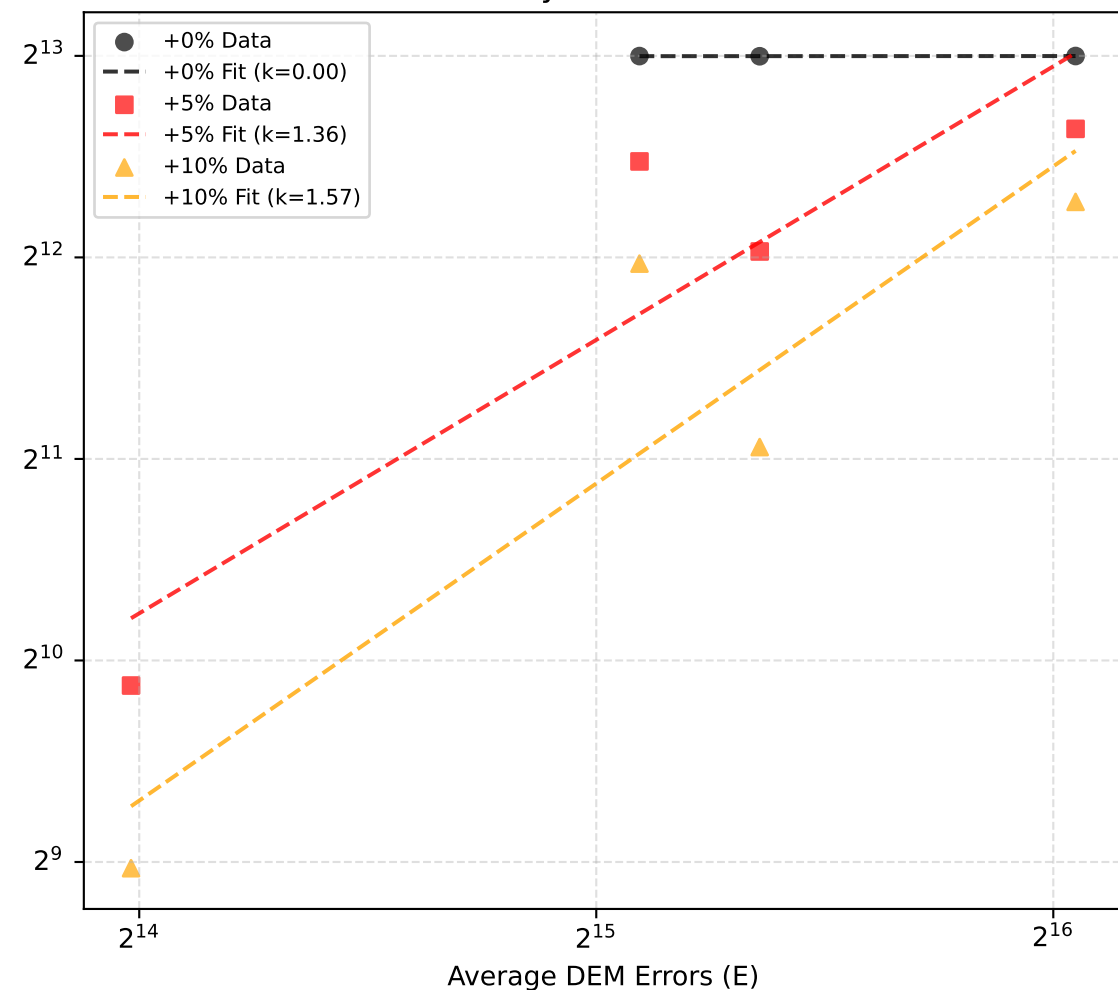
Bicycle Codes
