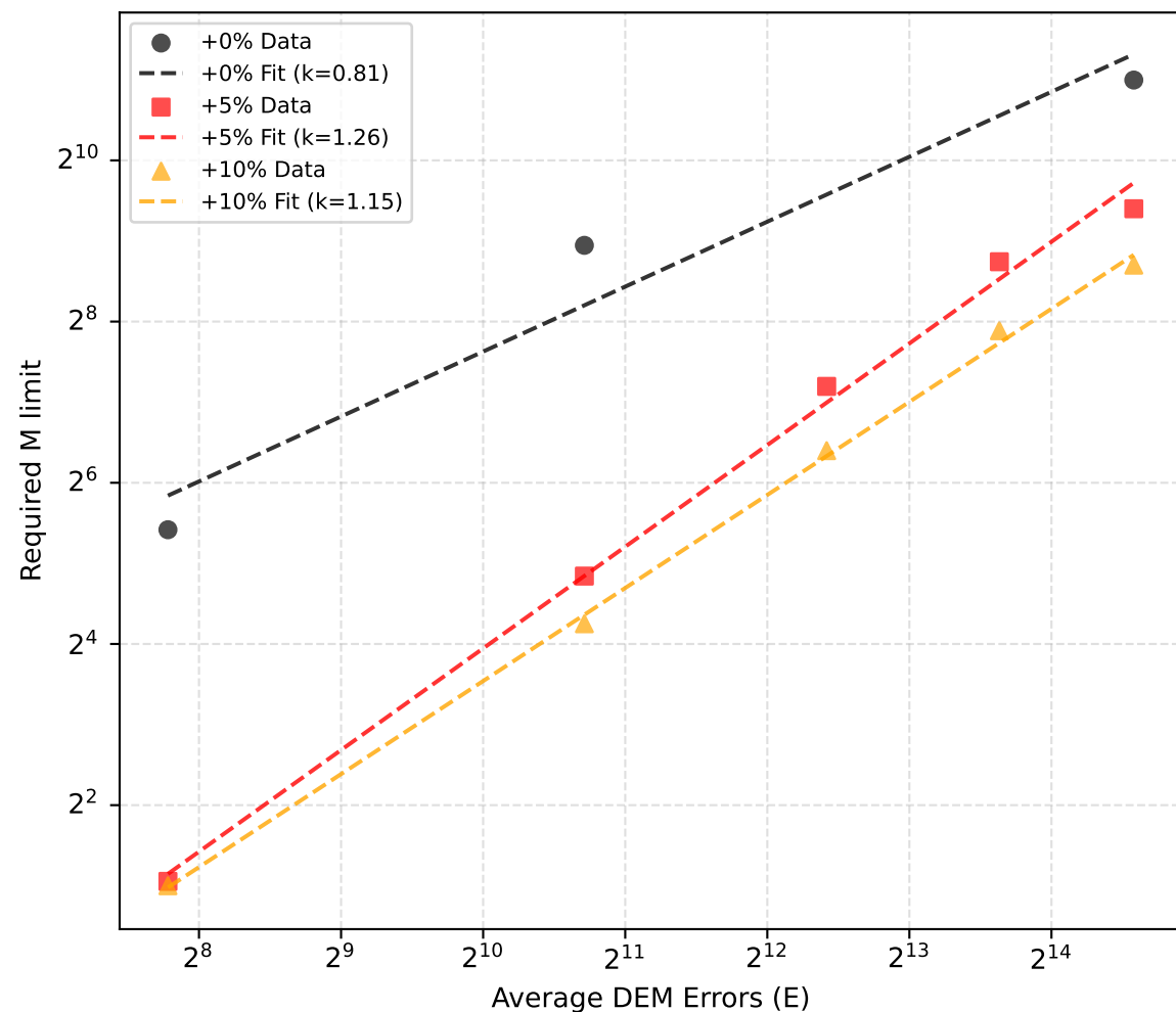
Surface Codes
