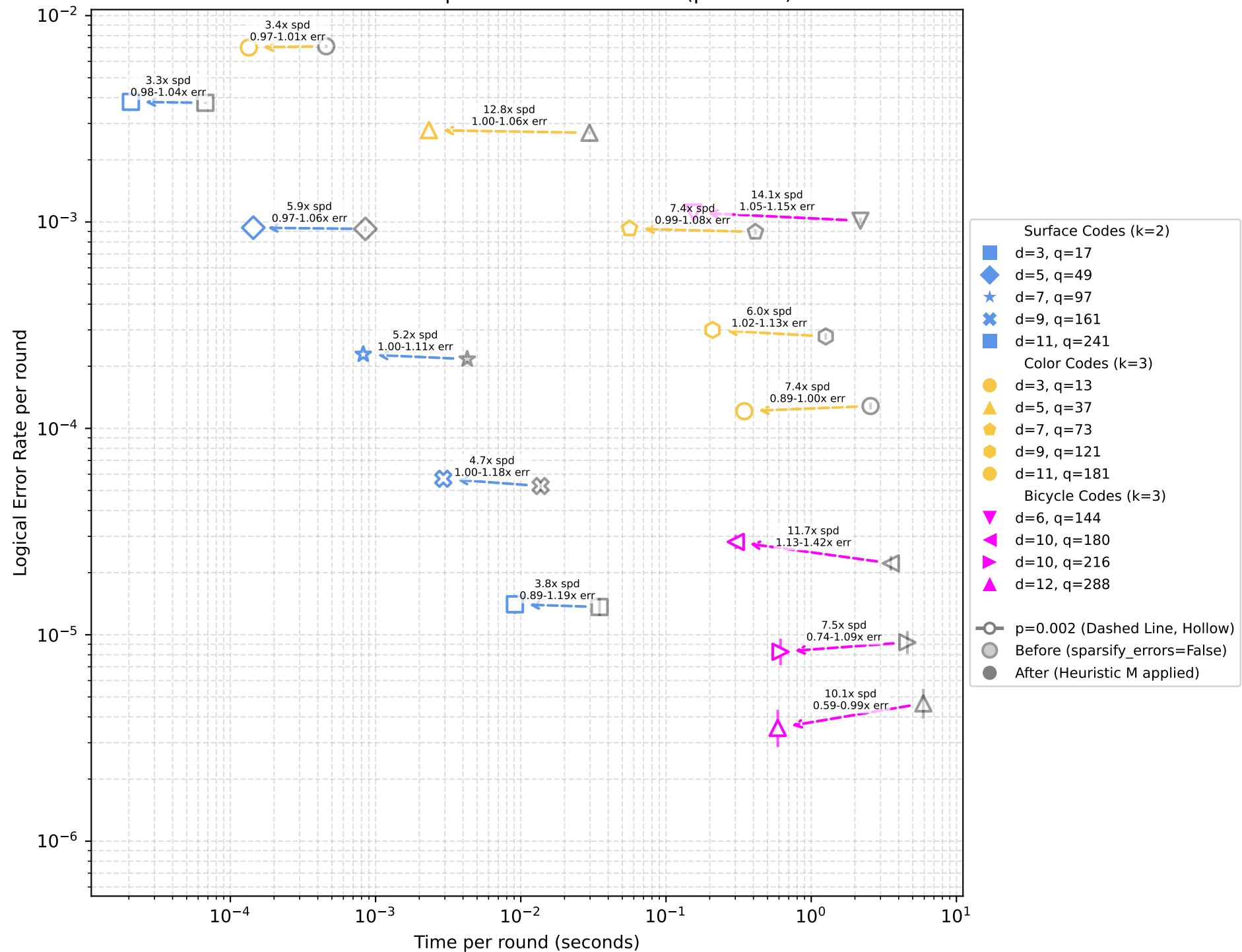
Before vs After: Sparsification Tradeoffs ( p=0.002 )
