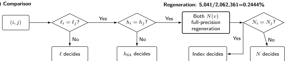
Figure 3: Storage format for bit lengths and leading bits and comparison paths. Different bit lengths or leading 64 bits determine the order from retained pairs alone. When both agree, full-precision norms are regenerated from compressed candidates. The regeneration rate shown is observed in the fixed-key timing test; comparison correctness does not depend on this frequency.
