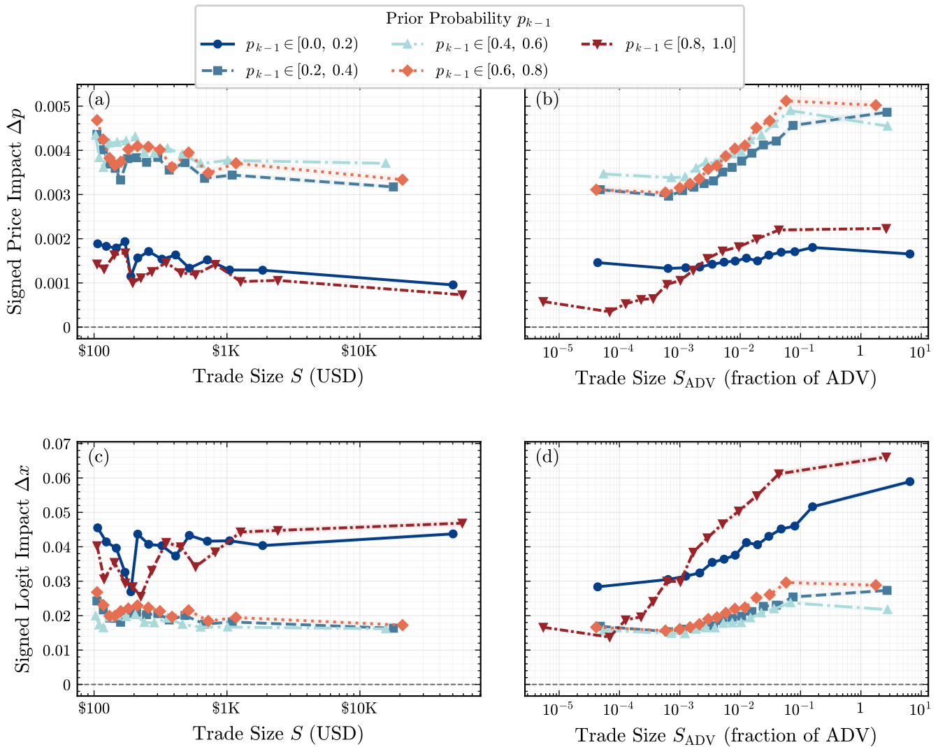
Mean Market Impact Conditional on Prior Probability Level p_{k-1} (Trade Size \geq \$100 )
