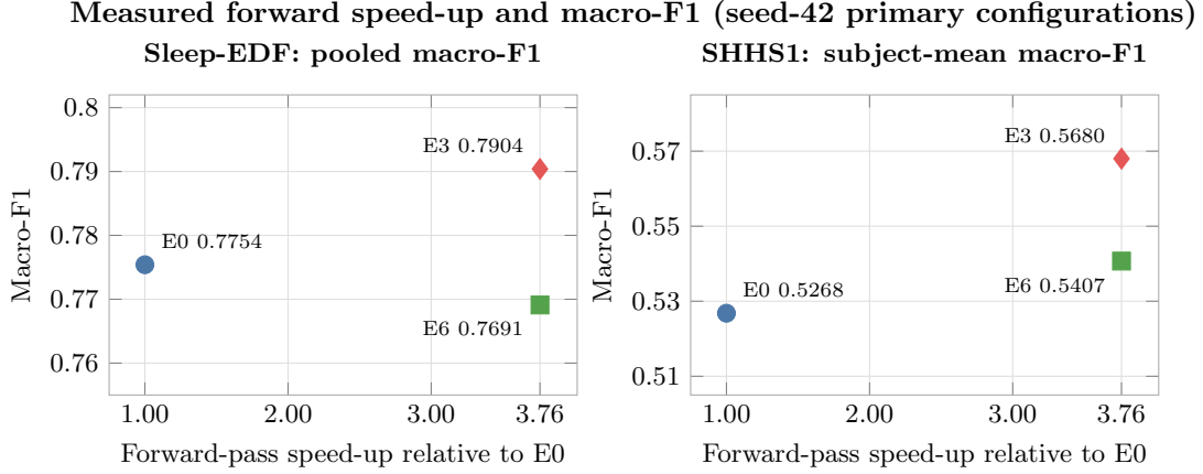
Figure 2. Measured forward speed-up and aggregate macro-F1 for the locked primary seed-42 configurations. Only E0, E3 and E6 are shown. The left panel reports pooled Sleep-EDF macro-F1; the right reports subject-mean macro-F1 on the locked SHHS1 sample. Speed-up is relative to E0 in the fixed forward-pass benchmark. The plot was generated from archived aggregate results using an editable PGFPlots source; OpenAI Codex assisted with the plotting code.
