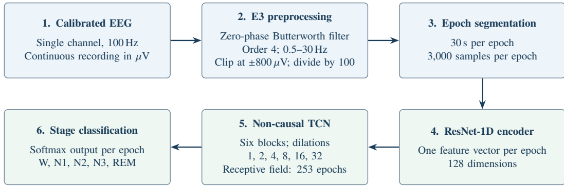
Figure 1. End-to-end processing pipeline for the proposed ResNet-1D-TCN single-channel sleep staging framework (E3 configuration). The raw continuous EEG signal is sequentially preprocessed (band-pass filtered, clipped, and scaled), segmented into 30 s epochs (3,000 samples), encoded into 128-dimensional feature vectors by a 1D-ResNet, and temporally modeled by a six-block non-causal TCN with a 253-epoch receptive field before final Softmax classification. The schematic was drawn in TikZ with OpenAI Codex assistance; it depicts processing steps, not measured signals or predictions.
