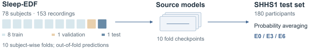
Figure 1. Model configurations and evaluation protocol. (a) E0 and E1 share a 15-CNN encoder: five branches for each of the current, previous and next epochs yield 75 features for a BiLSTM or TCN. E2, E3, E4 and E6 use separately fitted current-epoch ResNet-1D encoders and TCNs. ResNet numbers denote output channels; GAP is global average pooling. Both TCNs have six non-causal dilated blocks. E3 and E6 additionally clip at \pm 800 \mu\text{V} after band-pass filtering; E3 divides by 100, whereas E6 uses complete-record z-score statistics. (b) Sleep-EDF uses ten shared subject-wise folds, with eight for training, one for validation and one for testing per rotation. The primary SHHS1 evaluation compares E0, E3 and E6 on 180 participants, averaging class probabilities from ten source-fold checkpoints before selecting the predicted class, without target-domain model fitting. E6 uses unlabelled target-record statistics. E5 is an input-identity audit, not an additional performance configuration. Training settings and secondary analyses are described in the Methods and Supplement. The schematic was drawn with Matplotlib and OpenAI Codex assistance; the symbols represent architecture and fold roles, not measured signals or partition sizes.
