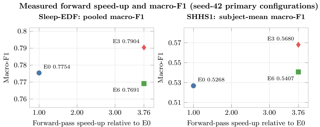
Figure 2. Measured forward speed-up and aggregate macro-F1 for the primary seed-42 configurations. Only E0, E3 and E6 are shown. The left panel reports pooled Sleep-EDF macro-F1; the right reports subject-mean macro-F1 on the SHHS1 sample. Speed-up is relative to E0 in the fixed forward-pass benchmark. The plot was generated from archived aggregate results using an editable PGFPlots source; OpenAI Codex assisted with the plotting code.
