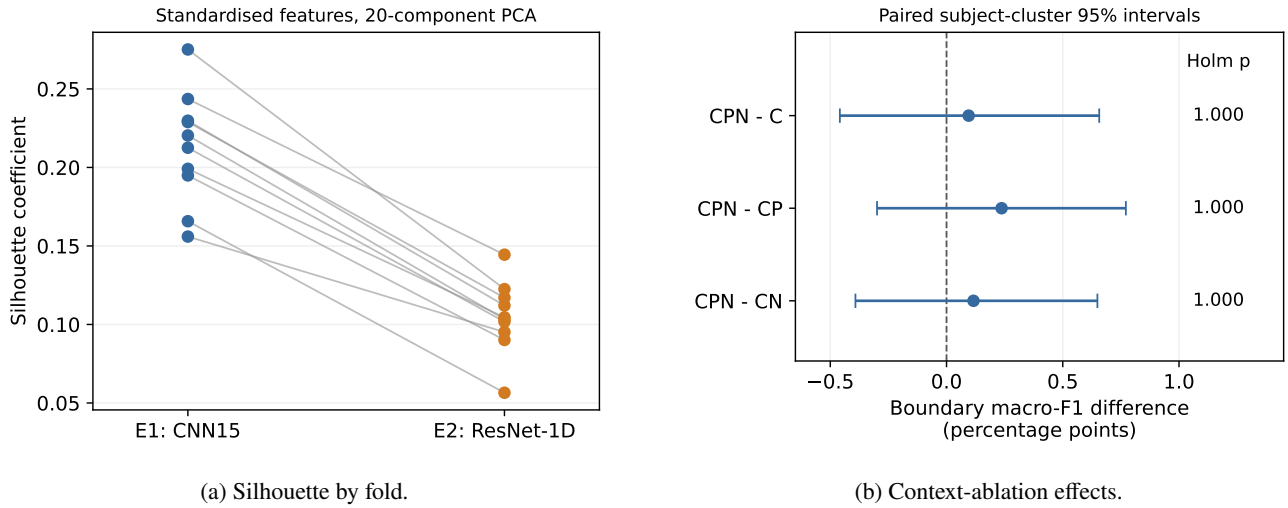
Figure S1: Supporting representation and context analyses. (a) Silhouette coefficients by test fold. (b) Paired 95% confidence intervals for pooled boundary macro-F1 differences: CPN minus C, CP and CN (Sleep-EDF, E1, seed 42). All intervals include zero; Holm-adjusted Wilcoxon p = 1.000 for each contrast. Plots were drawn from archived aggregates using repository code with OpenAI Codex assistance.
