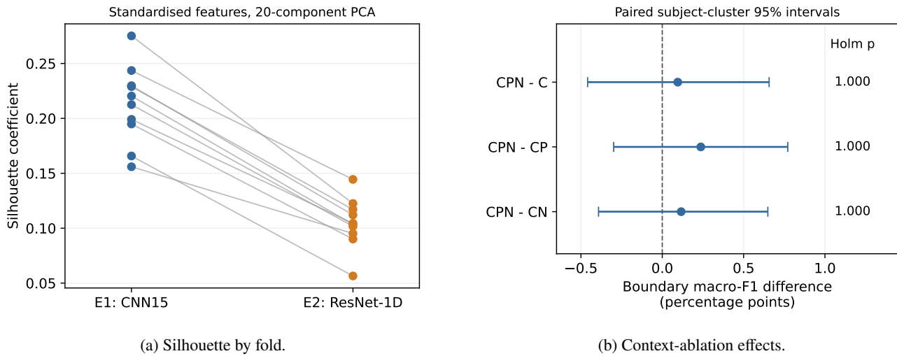
Figure S1: Supporting representation and context analyses. (a) Silhouette coefficients by test fold. (b) Context-ablation effects showing paired 95% confidence intervals of Boundary macro-F1 differences when ablating C/P/N context. The Holm p -values are 1.000 across all three Wilcoxon tests, demonstrating that removing this local temporal context does not significantly degrade boundary performance.
