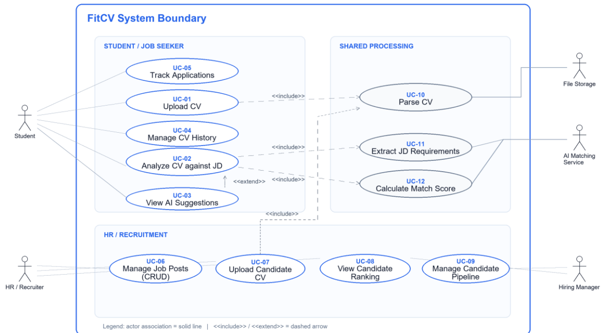
Figure 1. Overall Use-case Diagram for FitCV
