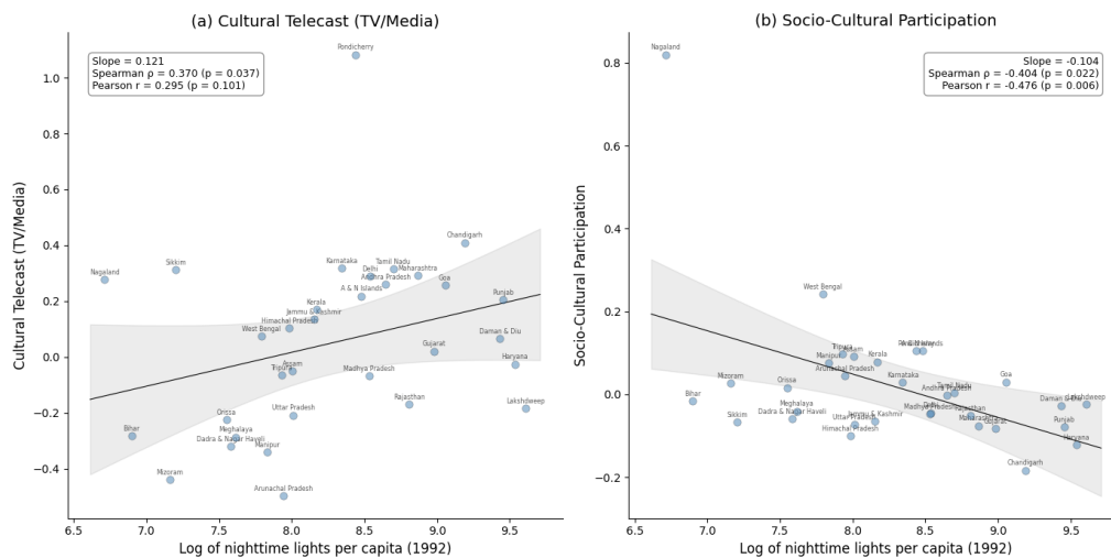
Figure 9: Relationship between nightlight luminosity and cultural participation across 32 Indian states and union territories. Notes: Each point represents one of the 32 Indian states and union territories. Panel (a) shows the bivariate relationship between log nighttime lights per capita and cultural telecast (TV/media); Panel (b) shows the relationship with socio-cultural participation. Solid line is the OLS regression; gray band shows the 95% confidence interval (t-distribution, 30 df). Annotations report regression slope, Spearman rank correlation, and Pearson correlation. Source: Nighttime lights from CCNL DMSP-OLS (Zhao et al., 2022). Cultural participation from NSS 47th Round (July–December 1991). See Spatial culture notebook for source code.
