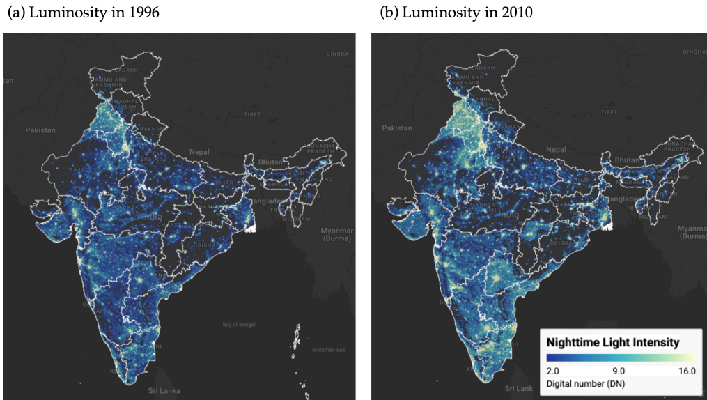
Figure 1: Regional luminosity in India: 1996 vs 2010
