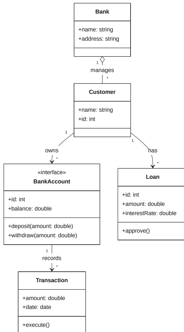
Figure 13.1: Class diagram of a bank system.
