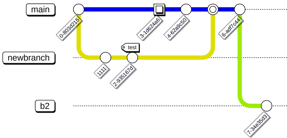
Figure 13.4: Graph of a Git repository.
