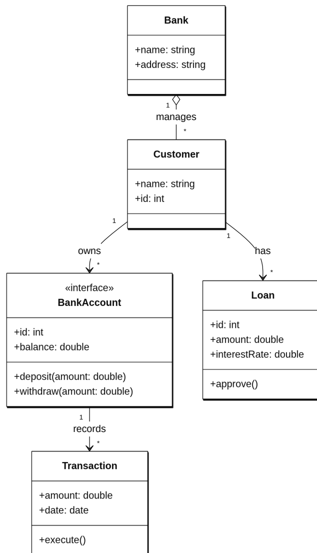
Figure 13.1: Class diagram of a bank system.
