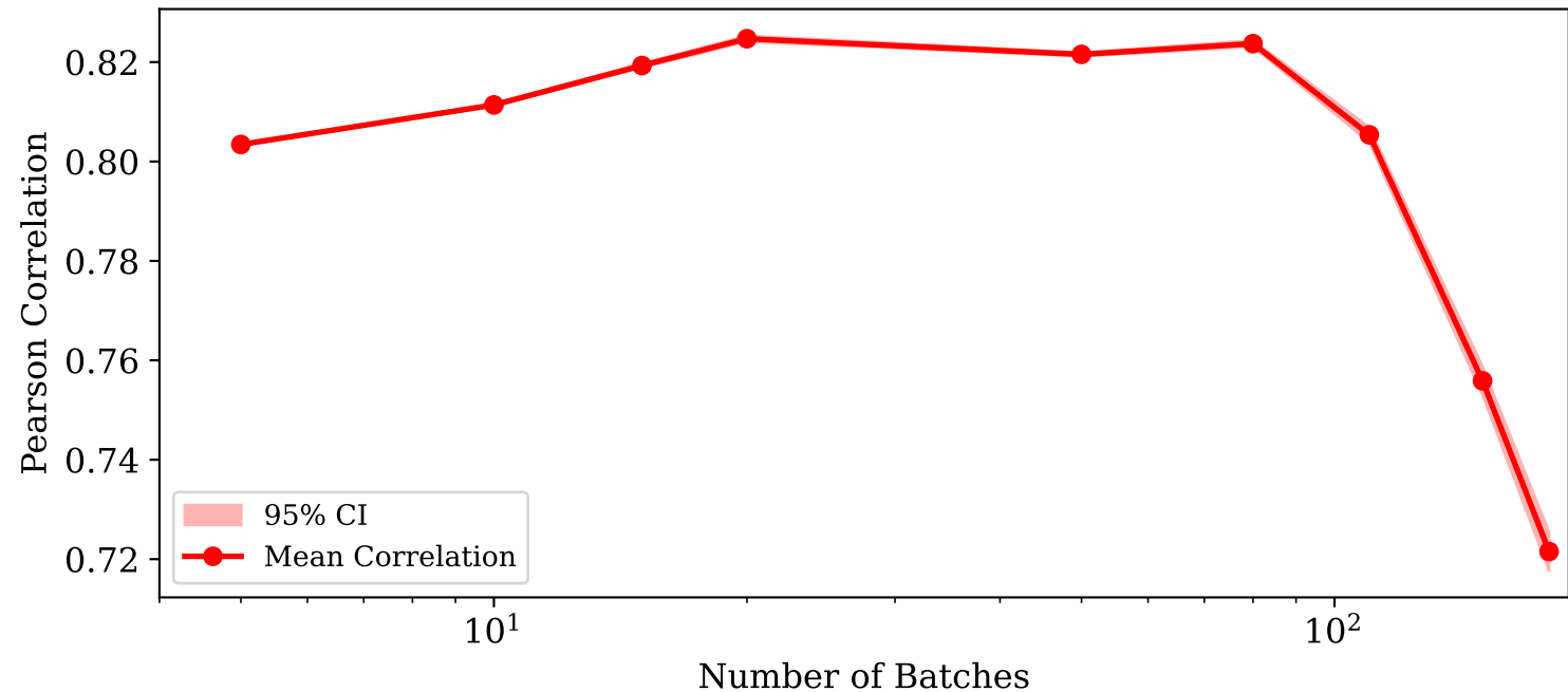
Effect of N° of Batches on SBert Performance
