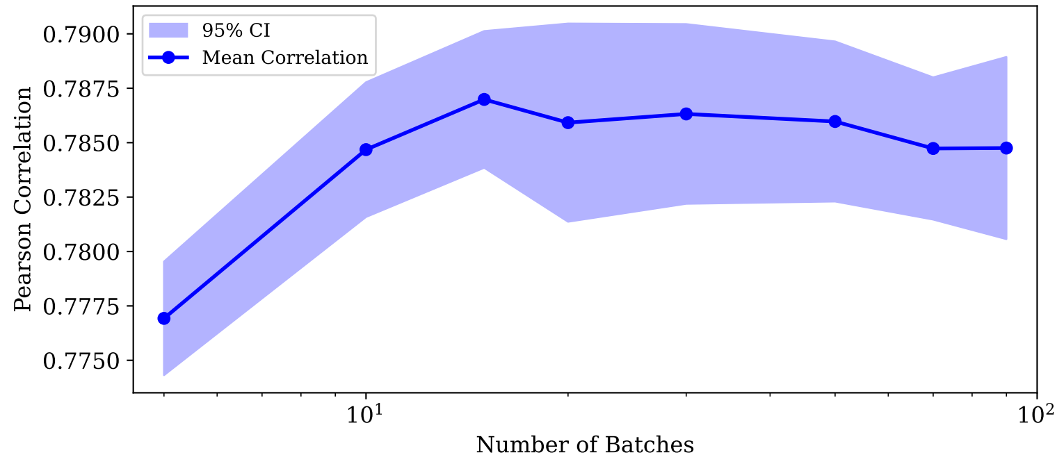
Effect of N° of Batches on Batches on SimCSE Performance
