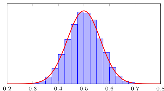
Distribution of \bar{X} and Gaussian( \frac{1}{2}, \frac{1}{\sqrt{240}} )
