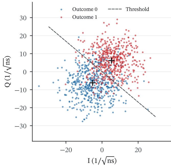
Fridge output at 6.5 GHz · 100 \mu s integration
