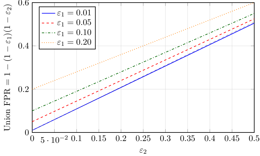
Figure 1: Union false positive rate \varepsilon = 1 - (1 - \varepsilon_1)(1 - \varepsilon_2) as a function of \varepsilon_2 for several fixed values of \varepsilon_1 . The thin dashed gray line shows the additive approximation \varepsilon_1 + \varepsilon_2 for \varepsilon_1 = 0.01 ; for small rates, the union FPR is nearly additive, but the product term \varepsilon_1\varepsilon_2 becomes significant as rates grow. By De Morgan duality, the intersection FNR has the same functional form with \omega_i replacing \varepsilon_i .
