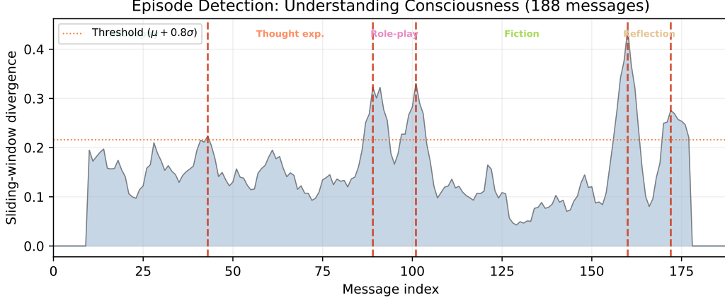
Figure 3: Sliding-window divergence signal for “Understanding Consciousness” (188 messages). Dashed vertical lines mark detected episode boundaries. Episode labels indicate the cognitive mode of each segment.
